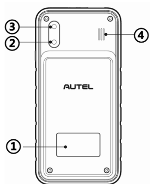
Figure 2-2 MaxiTPMS Tablet Back View
