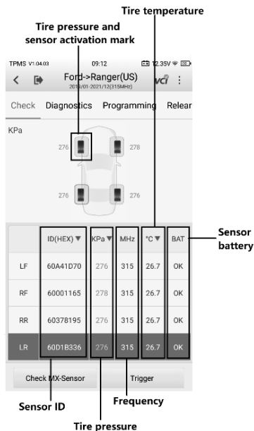
Figure 5-10 Check Screen
